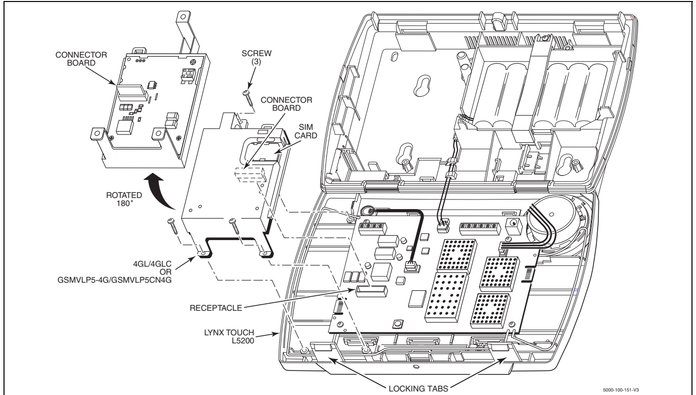
L5200 GSM Communications Installation
