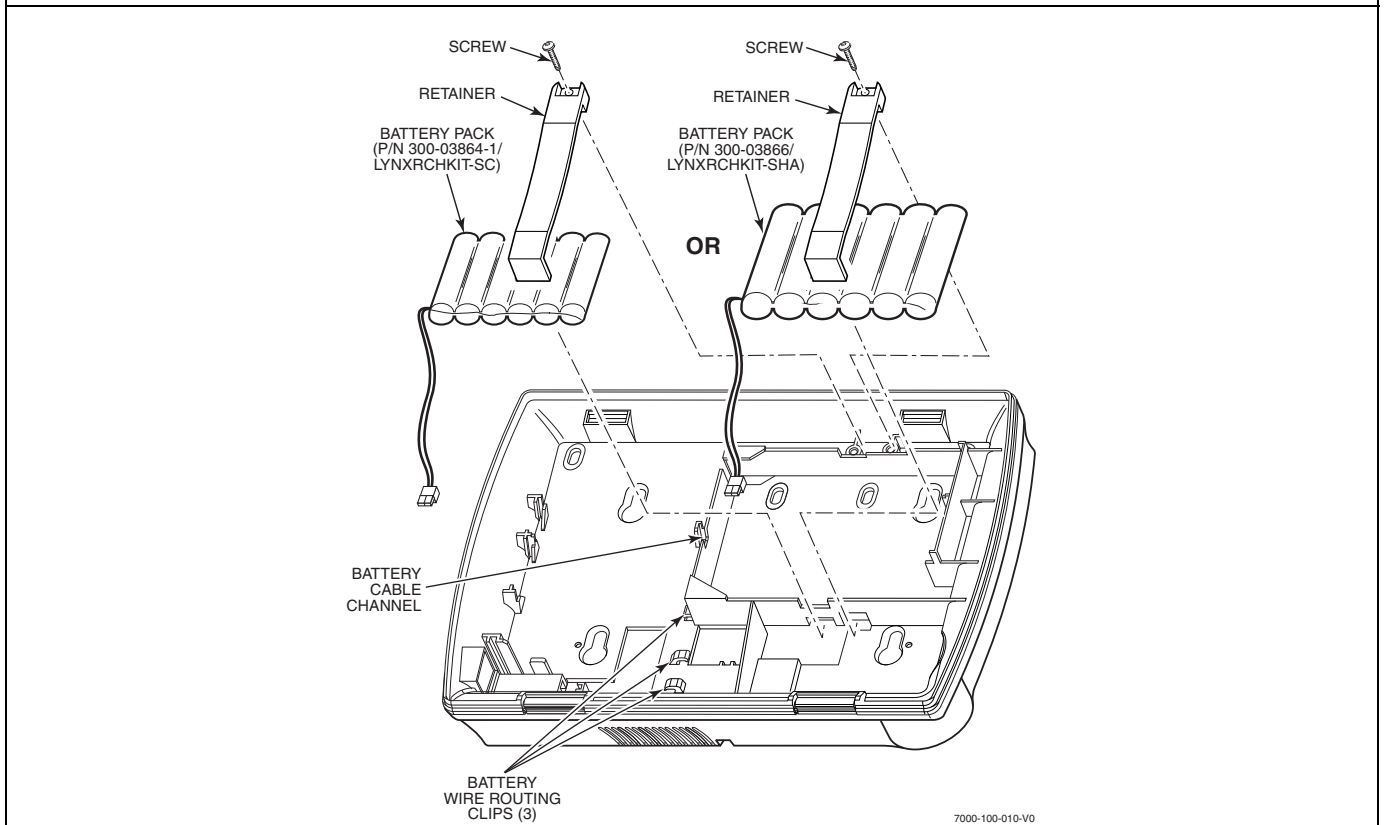
L7000 Battery Installation
