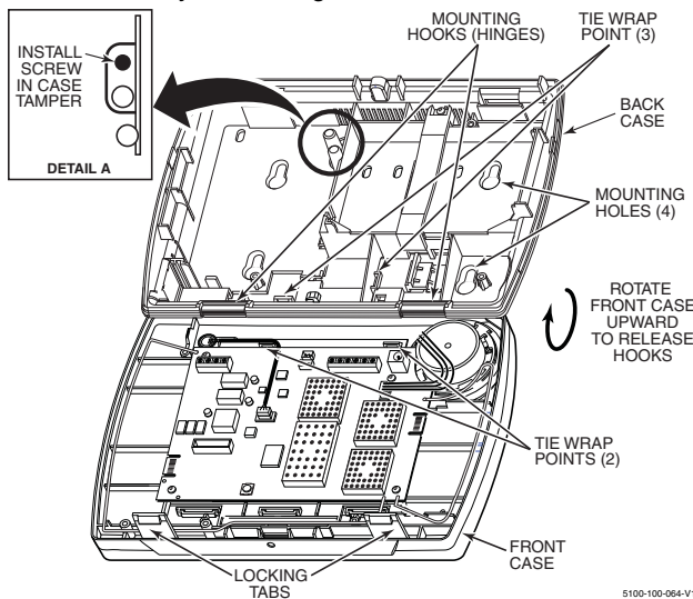
L5200 Wall Mounting
