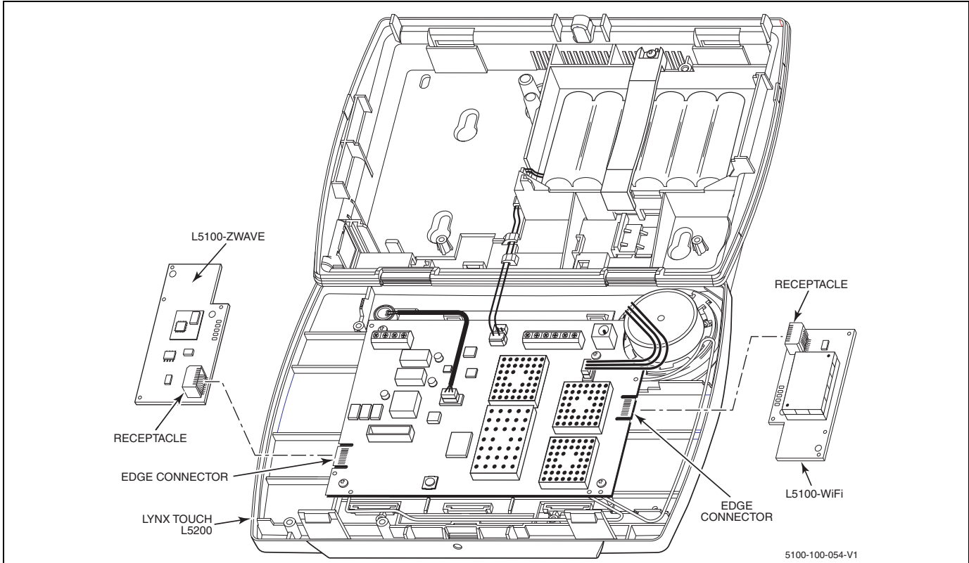
L5200 Z-Wave Automation & WiFi Communications Module Installation
