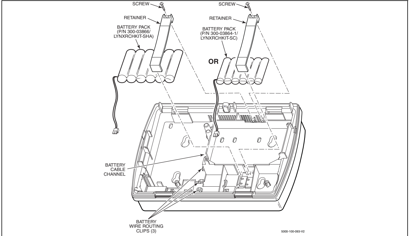
L5200 Battery Installation
