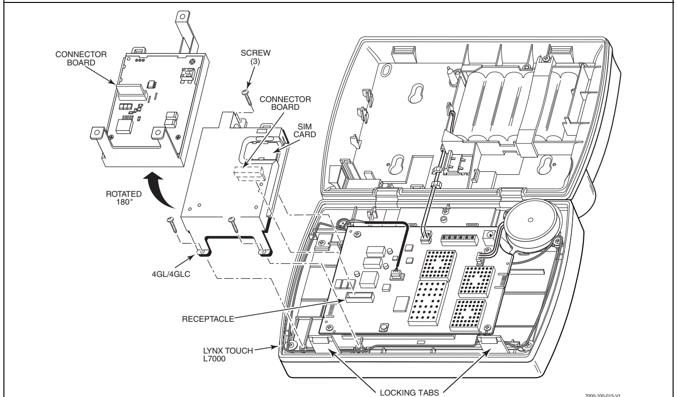
L7000 GSM Communications Module Installation
