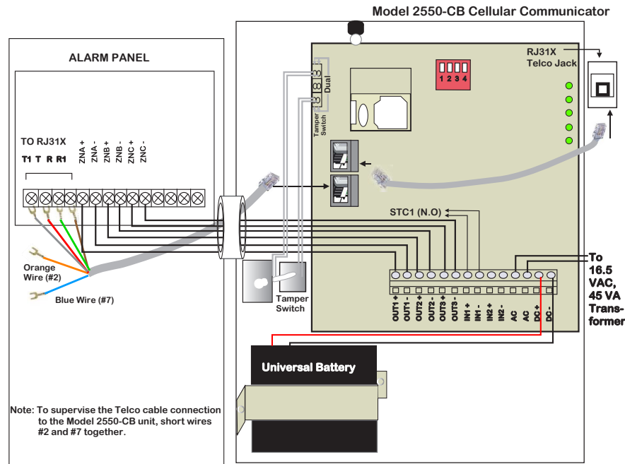
FIGURE 3: Example Connections Between the 2550-CB and the Alarm Panel. Refer to UL compliance section for specific UL wiring requirements and installation notes.
