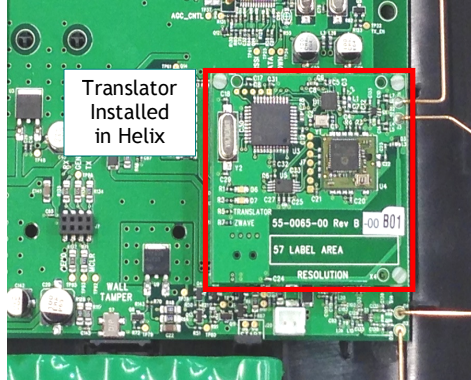
Expansion Slot 3
